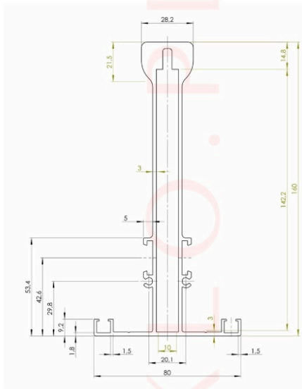
KROKIEW PR002
